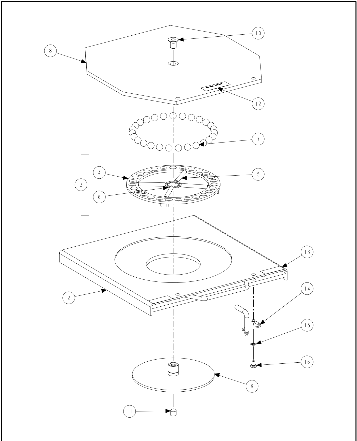
25-140-1 14 INCH TURNPLATE GAUGE REFER TO NEXT SHEET FOR PARTS DESCRIPTION LISTING
